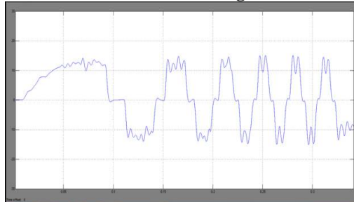
Motor Phase Current Ia
