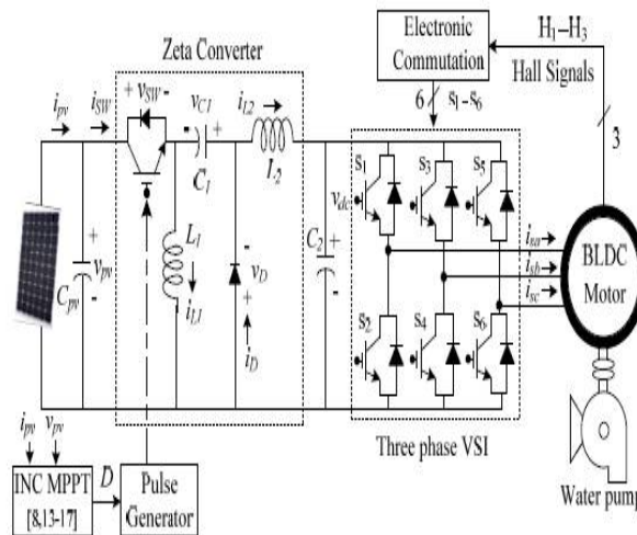
Fig.2. Proposed solar PV-zeta converter fed BLDC motor drive for water pump.
