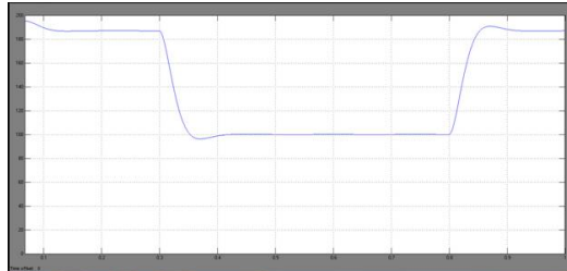
Vdc
