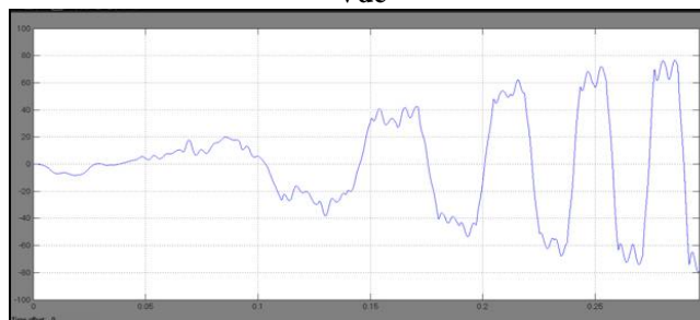
Motor Phase Voltage Ea
