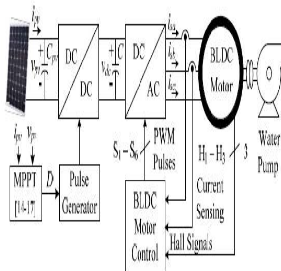
Fig. 1 Conventional SPV fed BLDC motor driven water pumping system.
