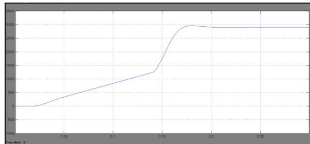
Motor Speed
